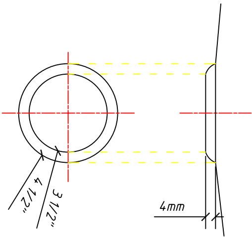
Cut-away view of drain opening
