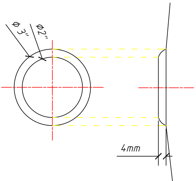
Cut-away view of drain opening
